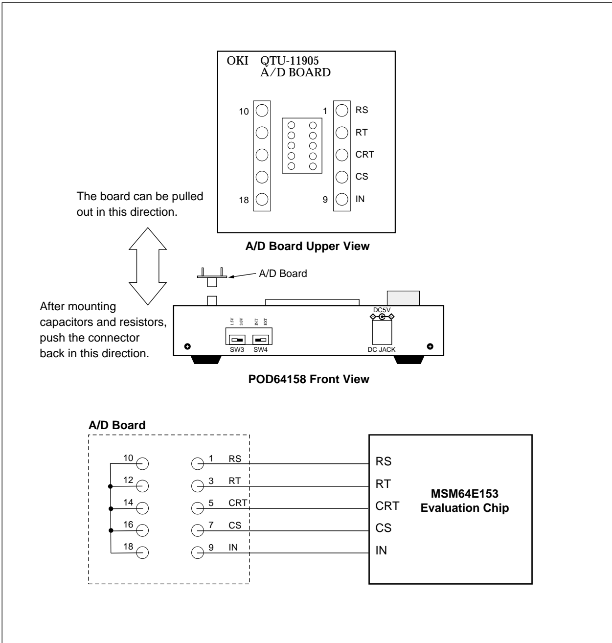
Figure 2-11. A/D Board
