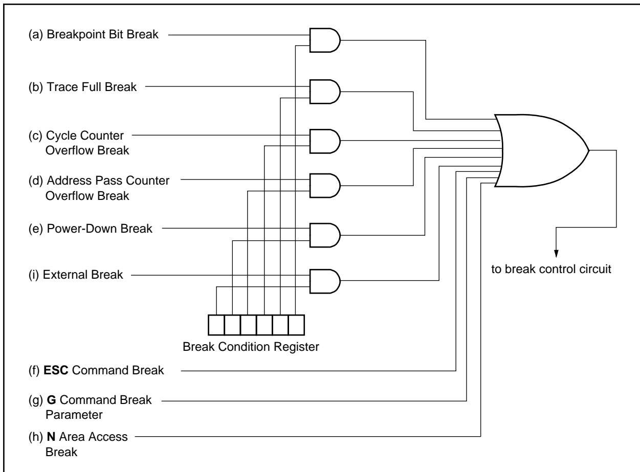
Figure 2-4. Break Masking
