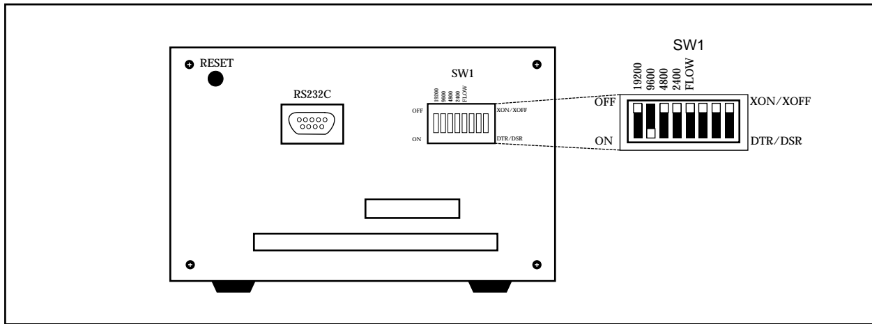
Figure 2-7. EASE-LP2 Dipswitches
