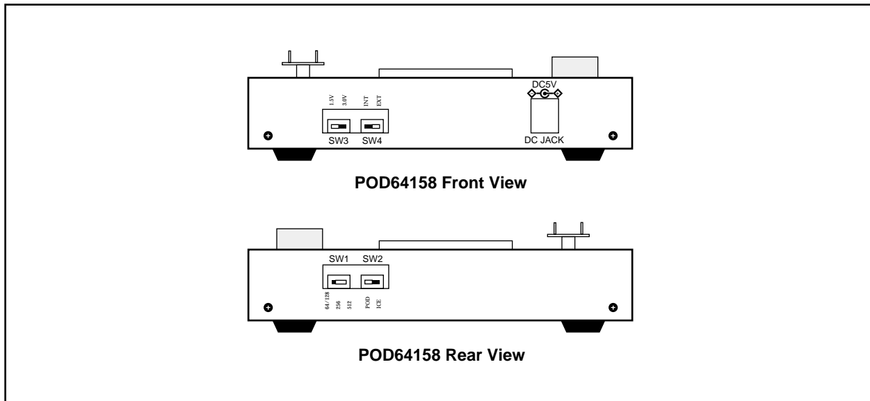
Figure 2-8. POD64158 Dipswitch
