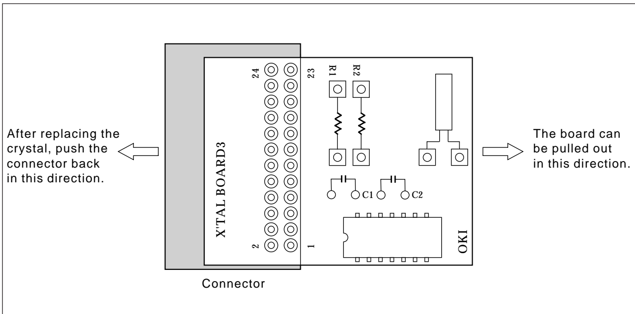
Figure 2-5. Crystal Board
