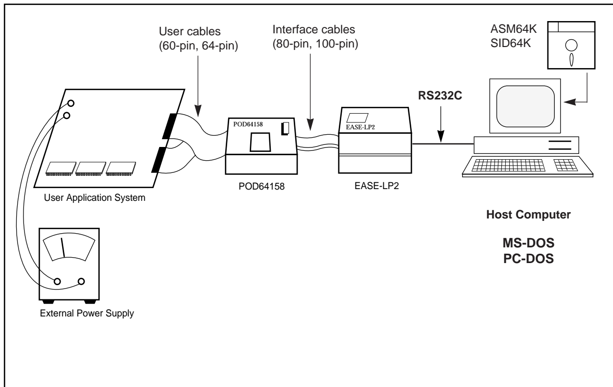
Figure 1-1. System Configuration in EASE-LP2 Mode
