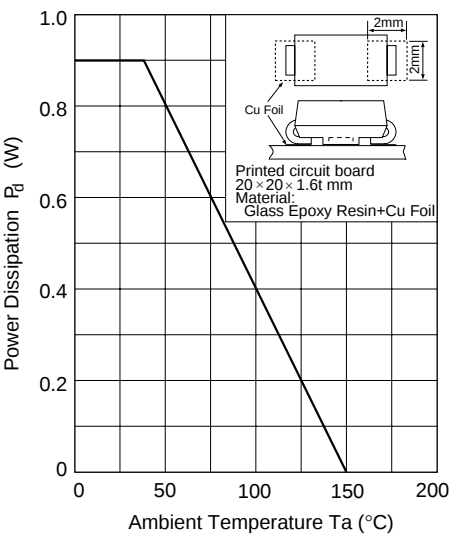
Fig.3 Power Dissipation Vs. Ambient Temperature
