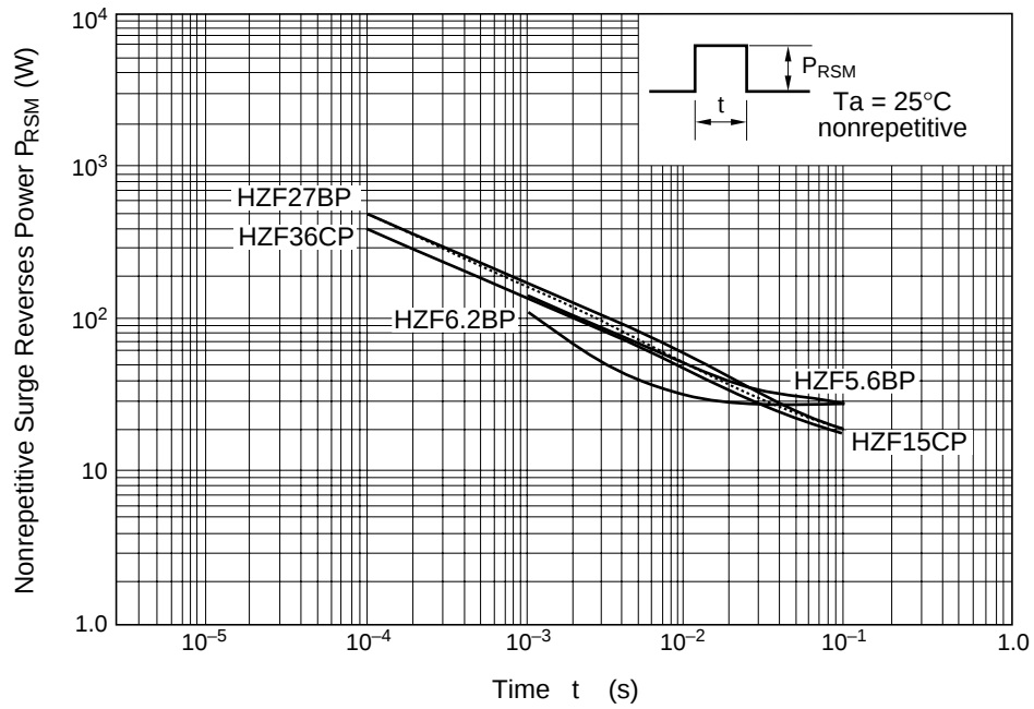
Fig.4 Surge Reverse Power Ratings (Reference only)
