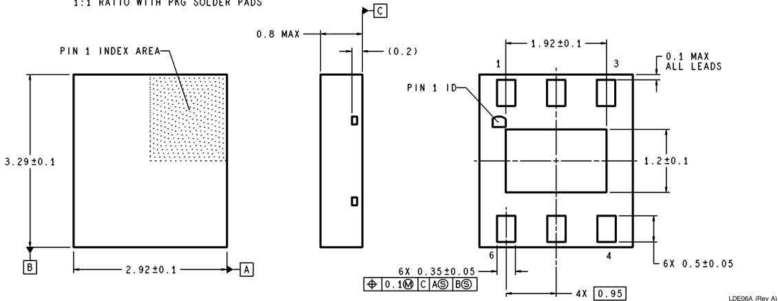
6-Lead LLP Package (LD) NS Package Number LDE06A
