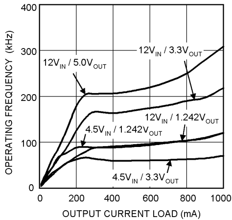
Operating Frequency vs Output Load Current
