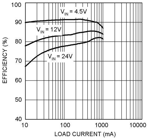
Efficiency vs Load Current (3.3 V OUT , 22µH)
