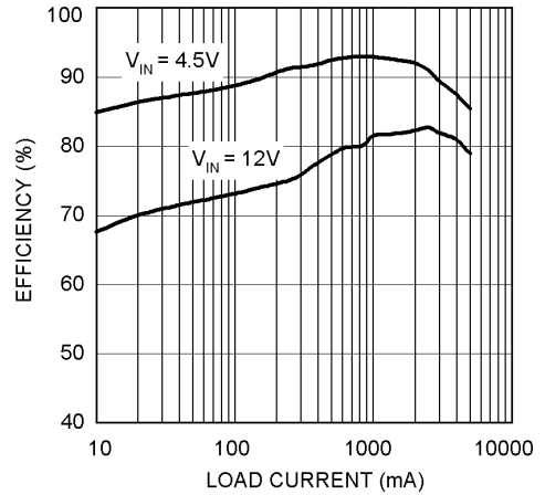
Efficiency vs Load Current (3.3 V OUT , 6.8µH)
