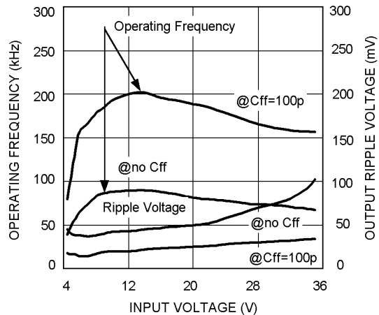
Feed-Forward Capacitor (C ff ) Effect
