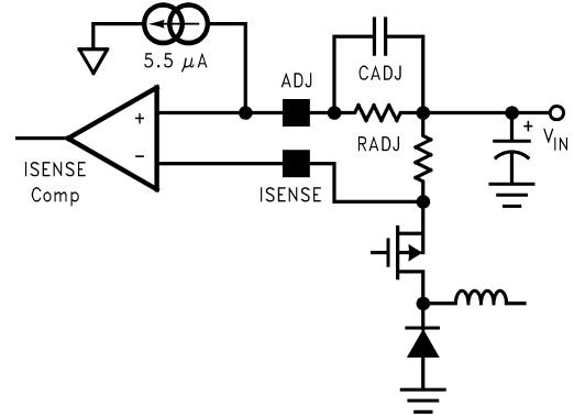
FIGURE 5. Current Sensing by External Resistor
