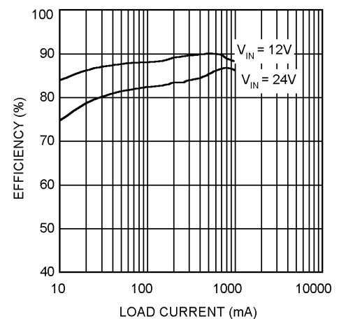
Efficiency vs Load Current (5.0 V OUT , 22µH)
