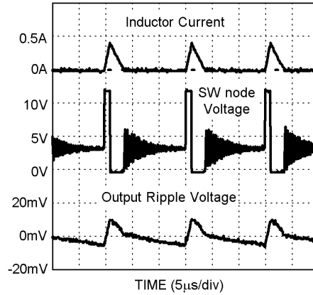
Discontinuous Mode Operation (12 V IN , 3.3 V OUT , 50mA Load, 22μH)
