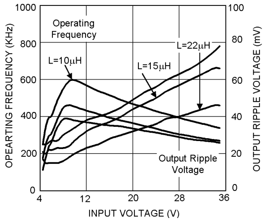
Operating Frequency and Output Ripple Voltage vs Input Voltage
