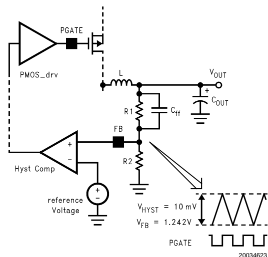
FIGURE 1. Hysteretic Window
