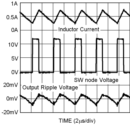
Continuous Mode Operation (12 V IN , 3.3 V OUT , 500mA Load, 22μH)
