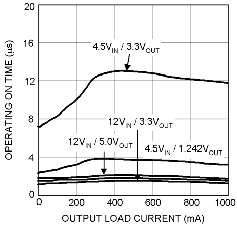
Operating ON Time vs Output Load Current
