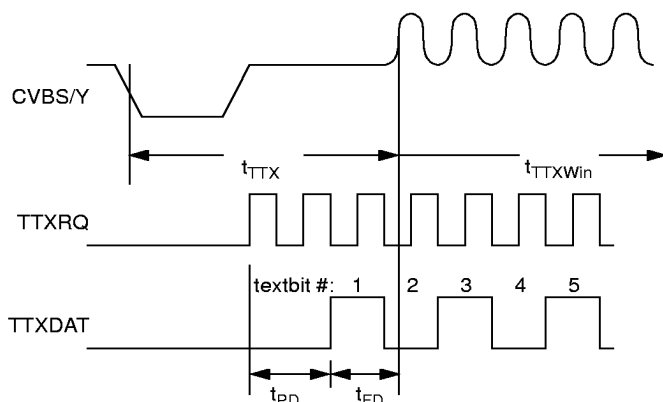
Figure 12. Teletext Timing (Pulsation Mode)
