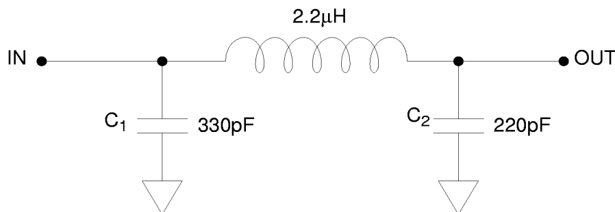
Figure 30. External Low Pass Filter C_2 should be chosen so that C_1 = C_2 + C_{\text{cable}}
