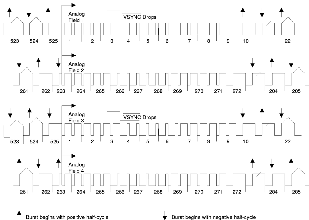
Figure 7. NTSC Video Interlaced Timing
