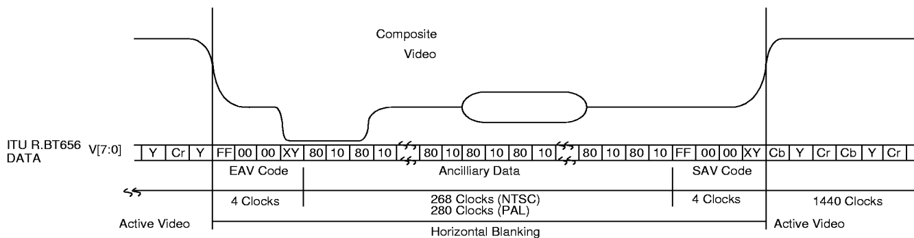
Figure 11. CCIR656 Input Mode Timing
