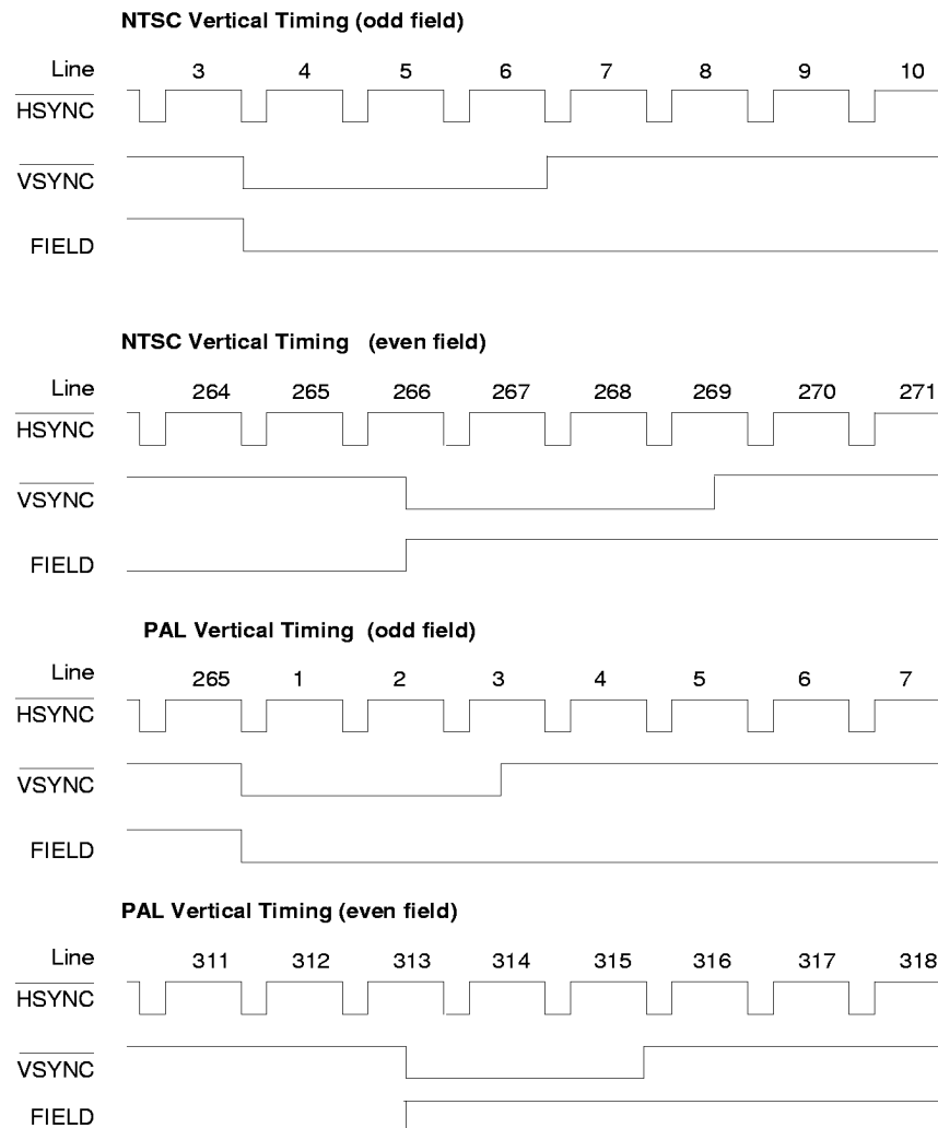
Figure 6. Vertical Timing
