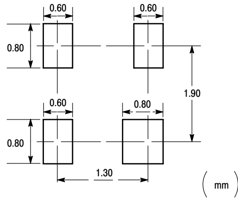
SC-82AB (SC70-4)
