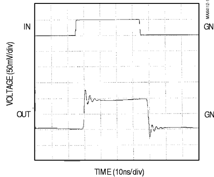
MAX4113/MAX4118/MAX4120 LARGE-SIGNAL PULSE RESPONSE ( A_{VCL} = +8 )
