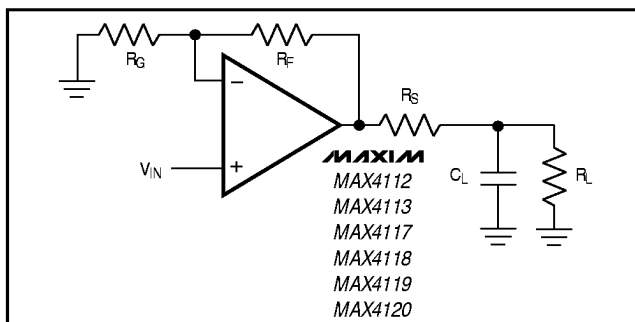
Figure 5a. Using an Isolation Resistor ( R_S ) for High Capacitive Loads
