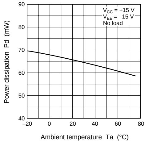
Power Dissipation vs. Ambient Temperature Characteristics
