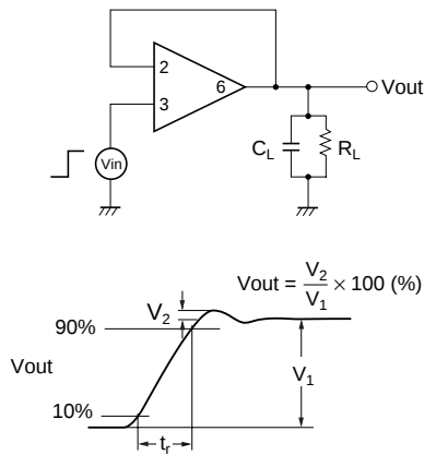
Impulse Response Characteristics Test Circuit
