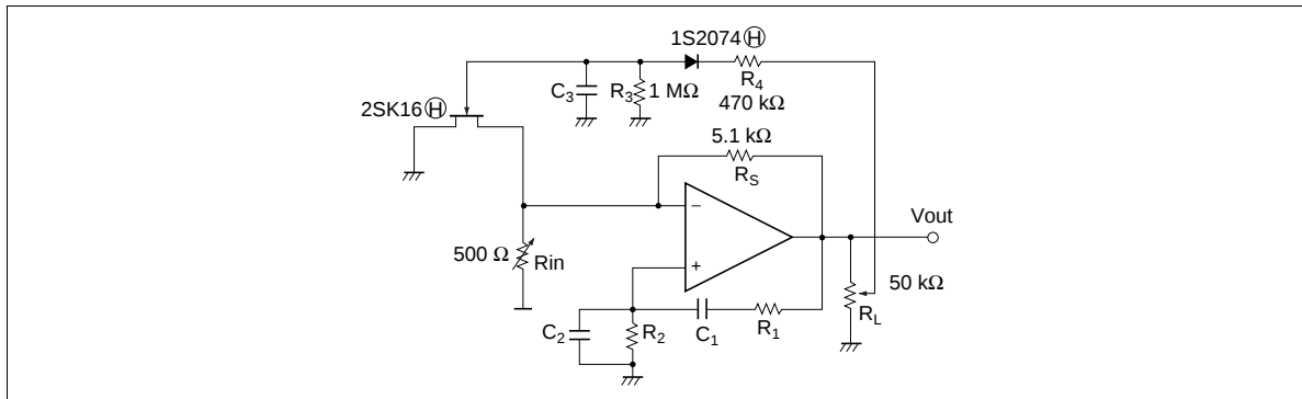
Figure 7 Wien Bridge Sine Wave Oscillator
