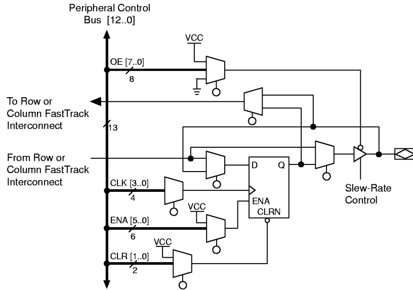
Figure 10. MAX 9000 IOC
