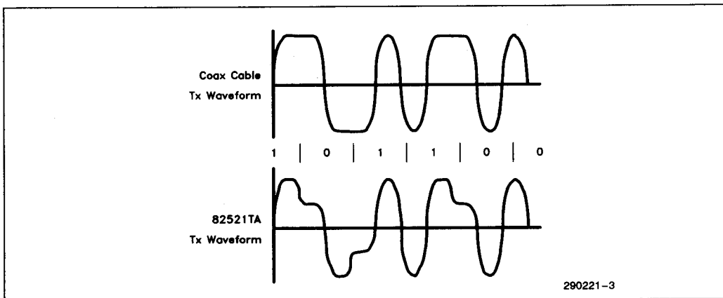
Figure 1. Effects of Predistortion
