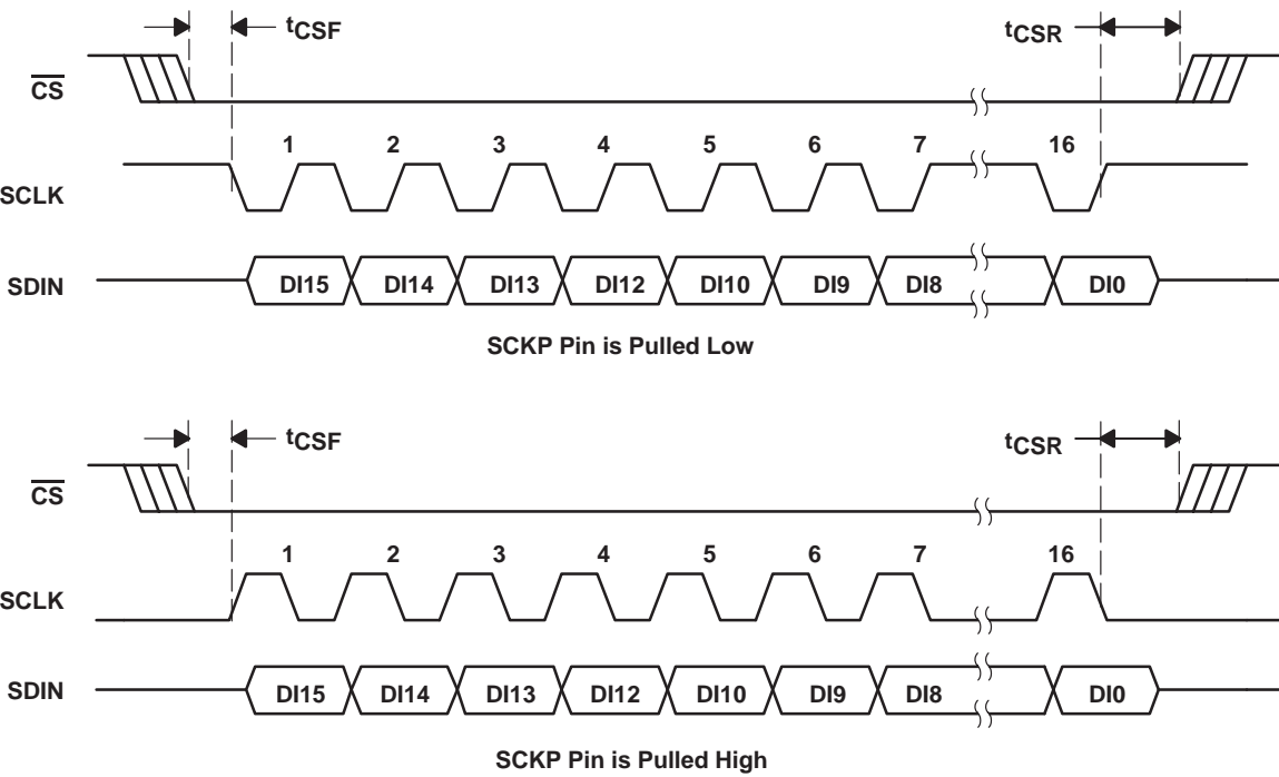
Figure 3. Serial Interface Timing Diagram
