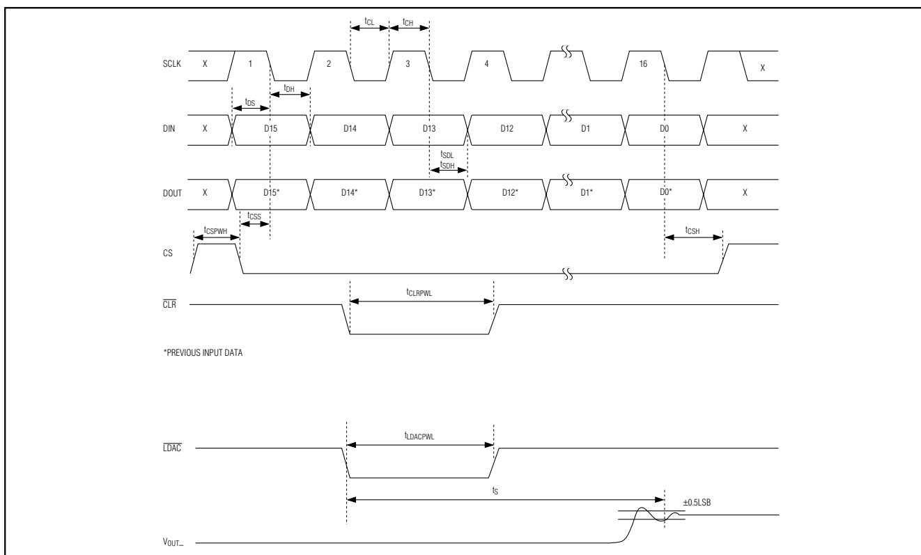
Figure 4. Timing Diagram
