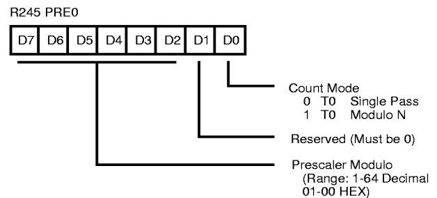
Figure 28. Prescaler 0 Register (F5 H : Write Only)
