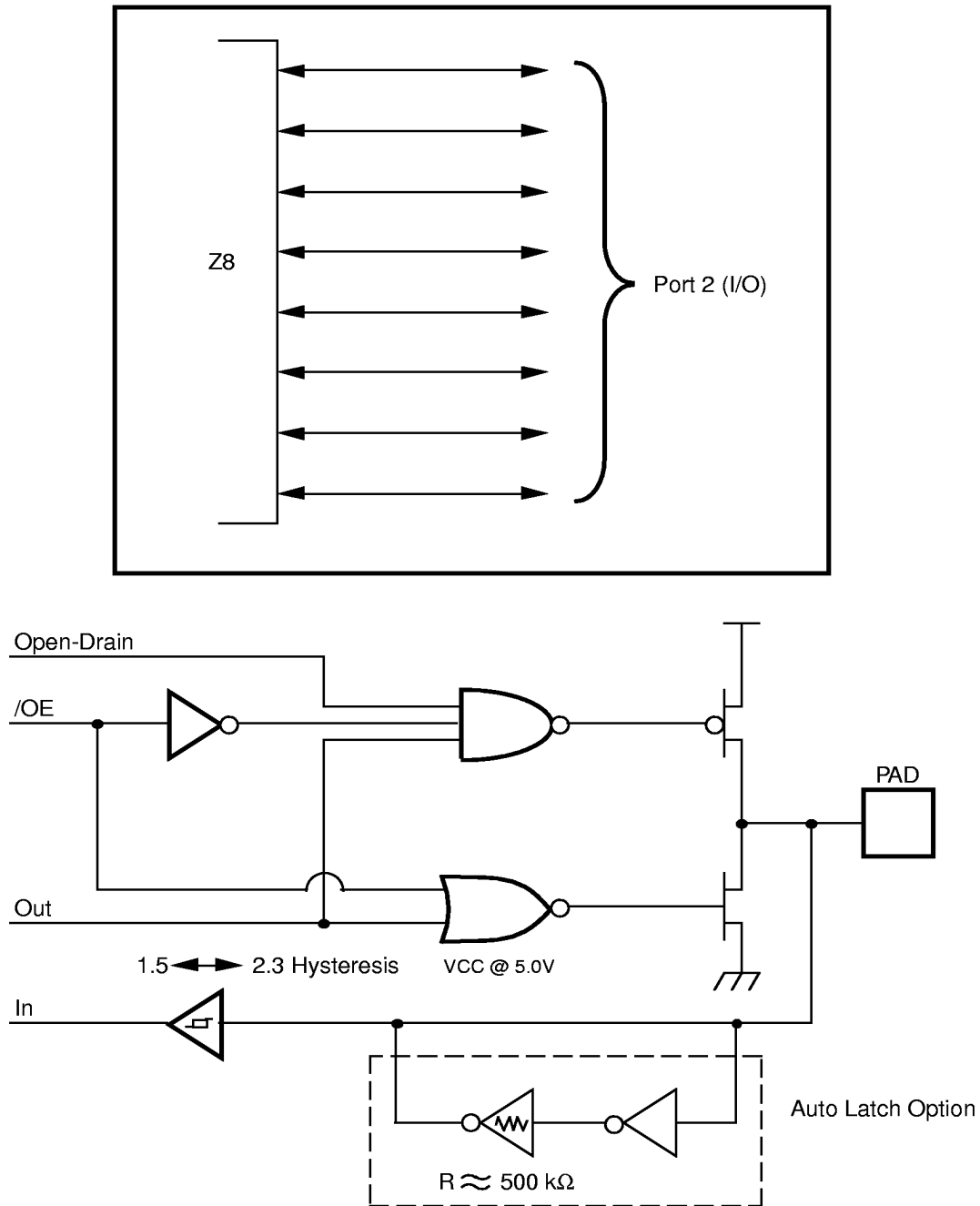
Figure 8. Port 2 Configuration
