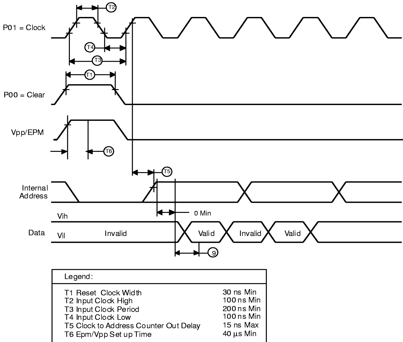
Figure 18. Z86E04/E08 Address Counter Waveform
