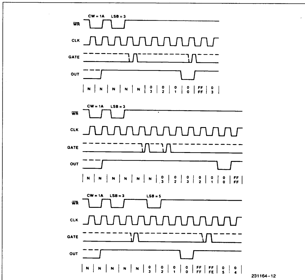
Figure 20. Mode 5
