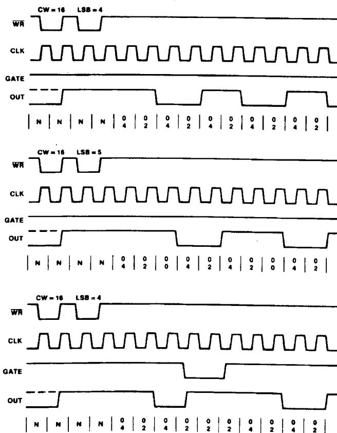
Figure 18. Mode 3
