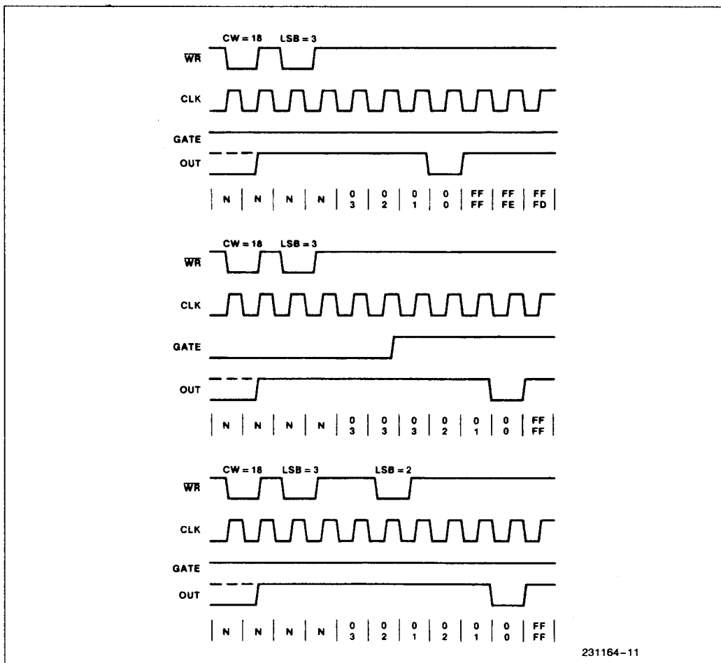
Figure 19. Mode 4
