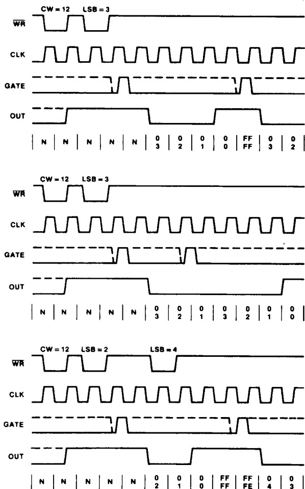
Figure 16. Mode 1
