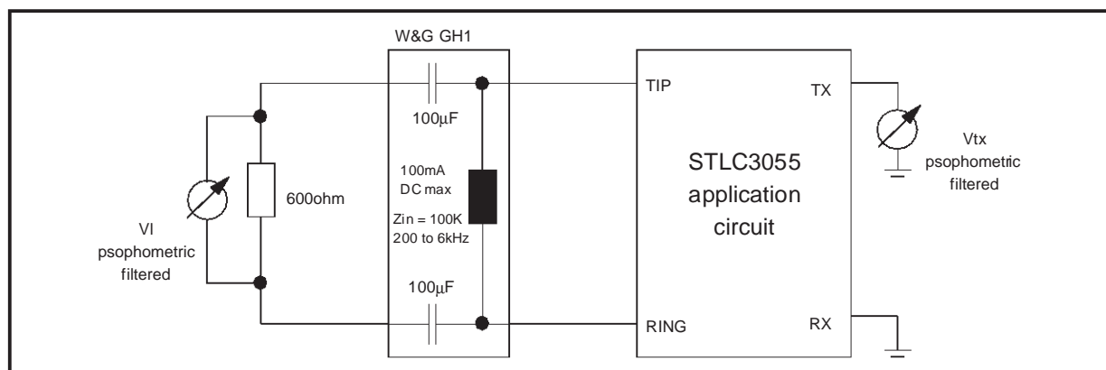
Figure A9. V2Wp and W4Wp: Idle channel psophometric noise at line and TX.
