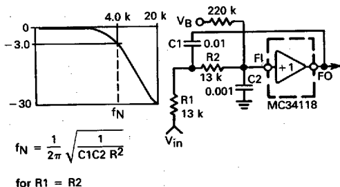
FIGURE 9 — LOW PASS FILTER
