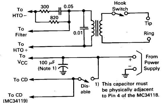
FIGURE 31 — OPERATING FROM A POWER SUPPLY
