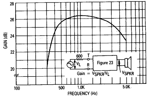
FIGURE 30 — RECEIVE GAIN
