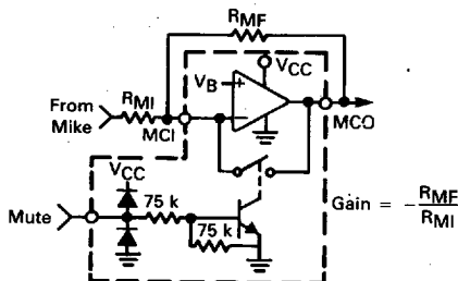
FIGURE 7 — MICROPHONE AMPLIFIER AND MUTE
