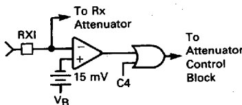
FIGURE 5 — DIAL TONE DETECTOR
