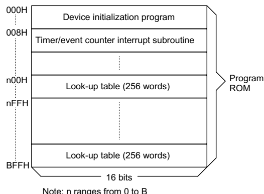
Program memory
