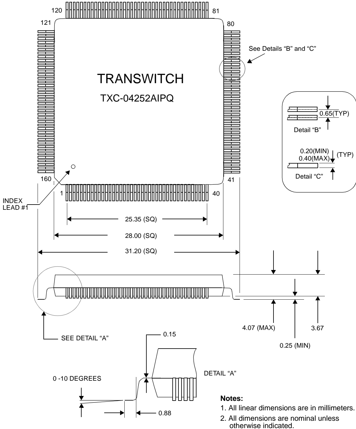
Figure 28. QE1M TXC-04252 160-Lead Plastic Quad Flat Package
