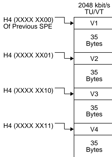
Figure 18. H4 Byte Floating VT Mode Bit Allocation
