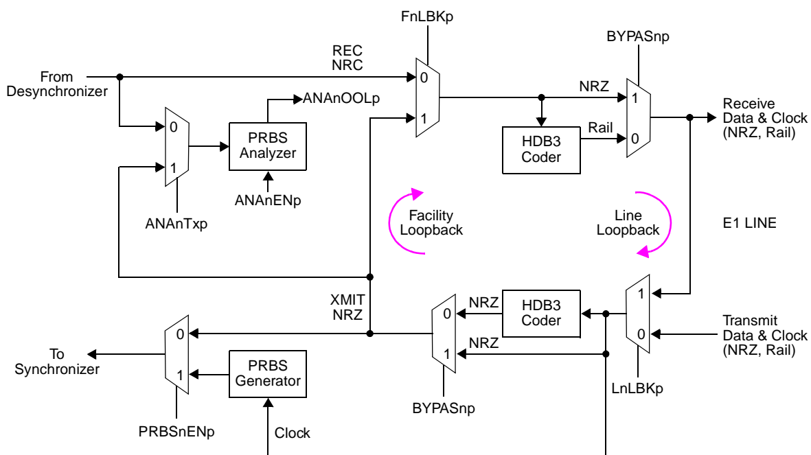
Figure 17. Facility and Line Loopbacks
