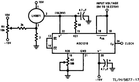
FIGURE 7. Offset and Full-Scale Adjustment Technique Using LH0071
