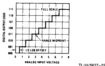
FIGURE 11. Transfer Characteristic Offset 1/2 LSB to Minimize Quantizing Uncertainty
