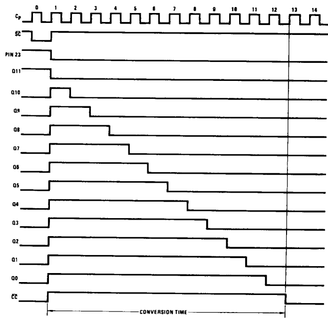
FIGURE 1c. Timing Diagram for V_{IN} = \text{Zero Scale}
