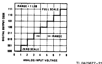
FIGURE 10. Quantization Uncertainty of a Perfect 3-Bit A/D
