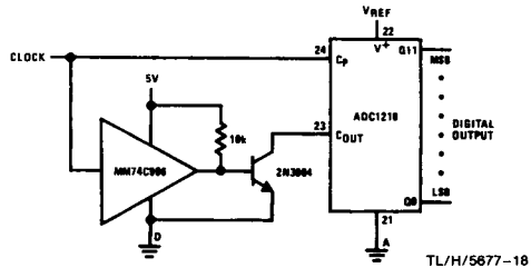
FIGURE 9. Conversion at 26 \mu s
