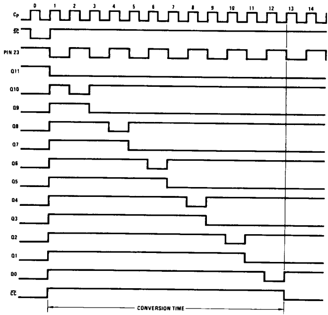
FIGURE 1d. Timing Diagram for V_{IN} = -3.4125V (010101010101)
