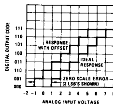
FIGURE 12. A/D Transfer Characteristic with Offset
