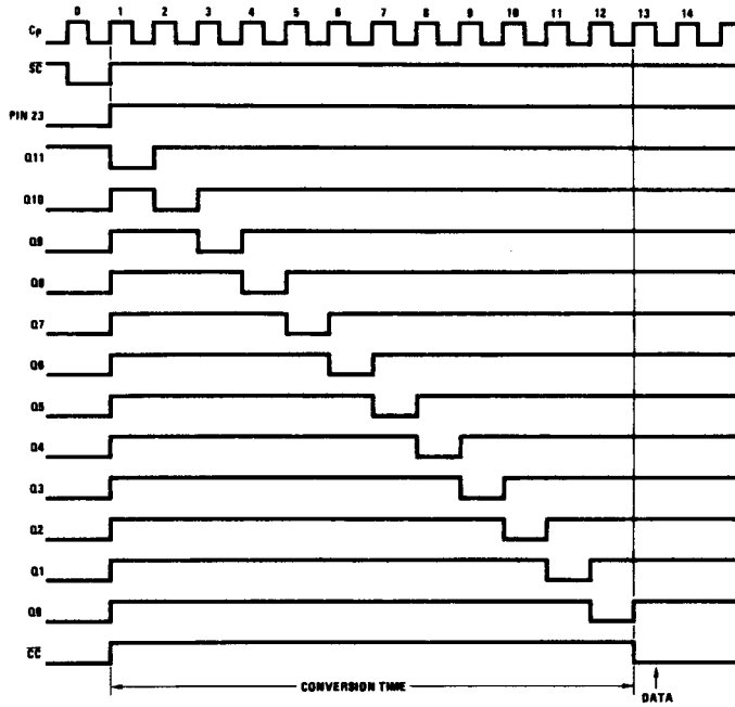
FIGURE 1b. Timing Diagram for V_{IN} = Full Scale Input
