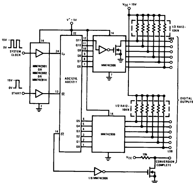
FIGURE 4. Interfacing an ADC1210, ADC1211 Running on V^+ < V_{CC} . Example: V^+ = 5V , V_{CC} = 15V
