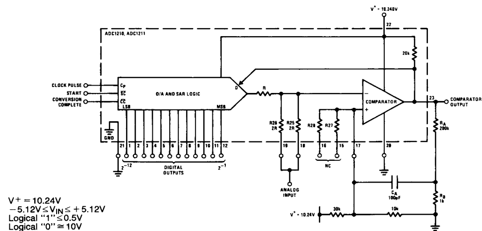
FIGURE 5c. Bipolar Input, Complementary Logic
