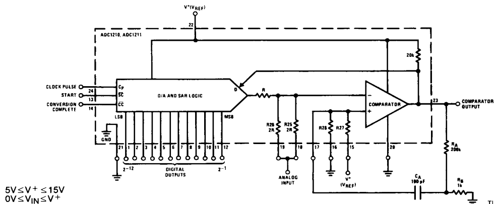
FIGURE 5a. Single Supply Configuration, Complementary Logic
