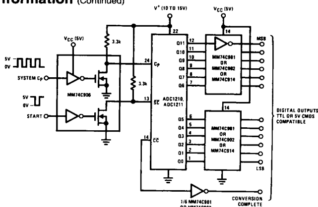
FIGURE 3. Interfacing an ADC1210, ADC1211 Running on V^+ > V_{CC} . Example: V^+ = 10.24V , System V_{CC} = 5V
