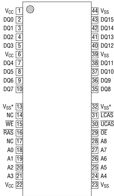
44/40-Pin Plastic TSOP (II) (K Type)
