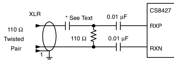
Figure 26. Transformerless Professional Input Circuit
