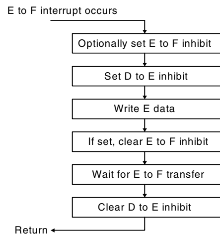
Figure 31. Flowchart for Writing the E Buffer
