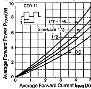
P F(AV) -I F(AV) Characteristics (CTG-11)
