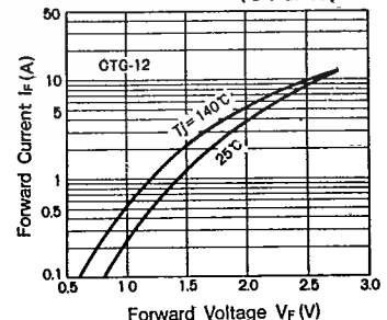
I F -V F Characteristics (CTG-12)
