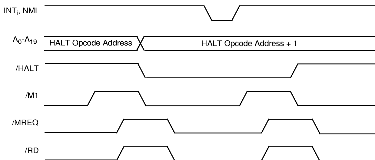
Figure 13. HALT Timing
