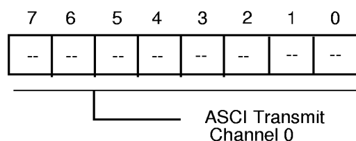
Figure 36. ASCI Register
