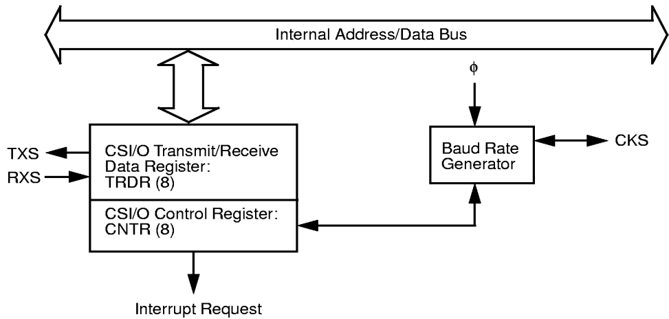
Figure 7. CSIO Block Diagram
