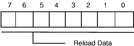
Figure 51. Timer Reload Register Channel 1L
