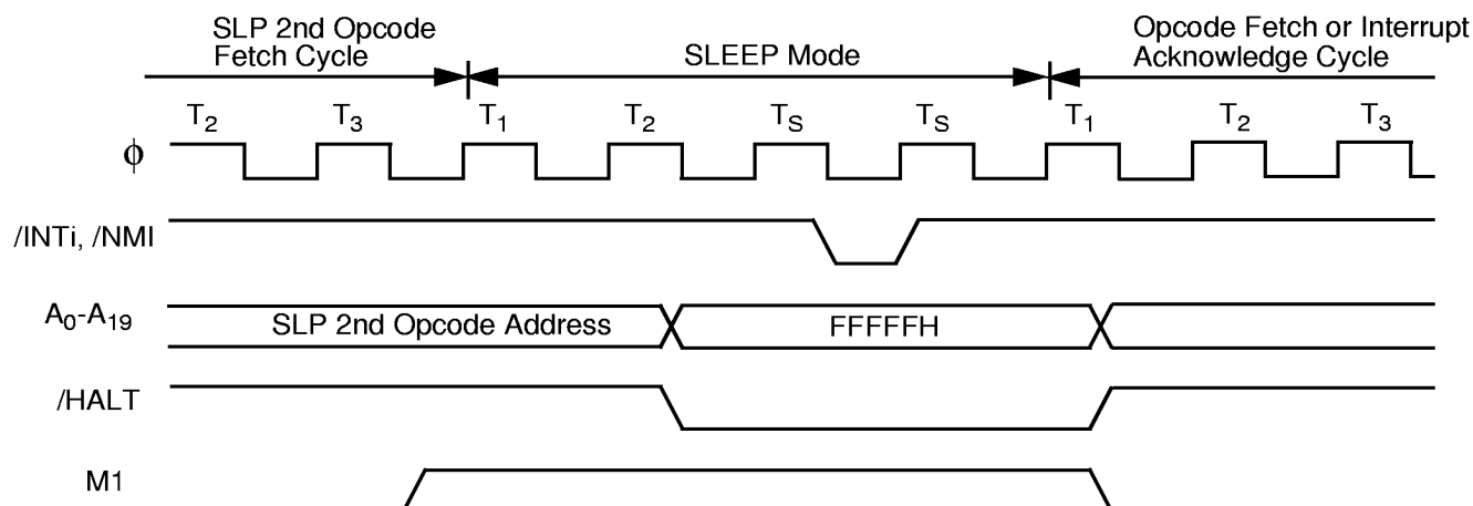
Figure 14. SLEEP Timing
