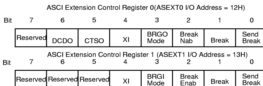
Figure 47. ASCI Extension Control Registers, Channel 0 and 1
