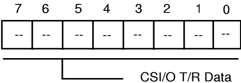
Figure 41. CSI/O Transmit/Receive Data Register 1R
