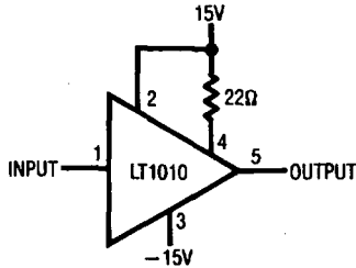
LT1010 Buffer†
