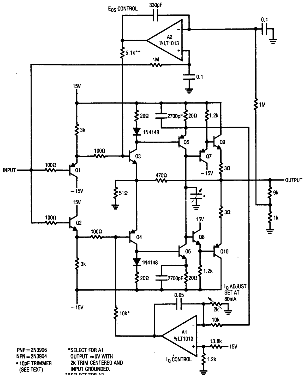
Wideband Discrete Buffer with Gain = 10†
