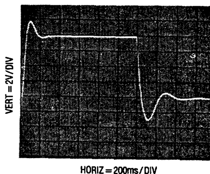
Figure 4's Settling Time (LT1088CD)
