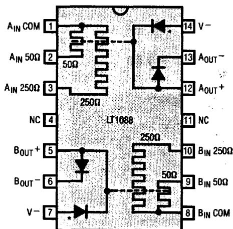
*DENOTES PARASITIC DIODE, SEE APPLICATIONS INFORMATION
