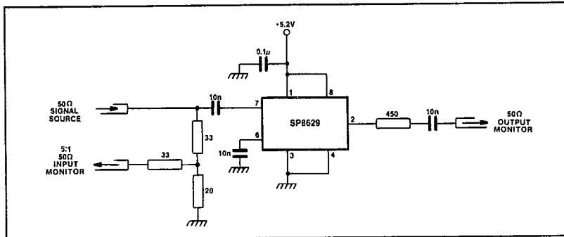
Fig.5 Test circuit
