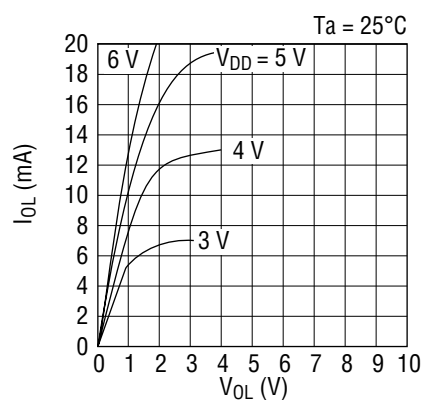
Typ. Current ( I_{OL} ) vs Voltage ( V_{OL} ) for Low State Output
