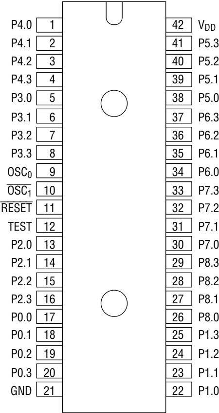
42-Pin Plastic DIP
