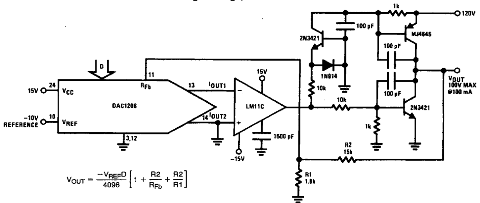
High Voltage, Power DAC
