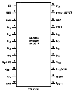
Dual-In-Line Package
