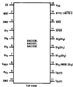
Dual-In-Line Package
