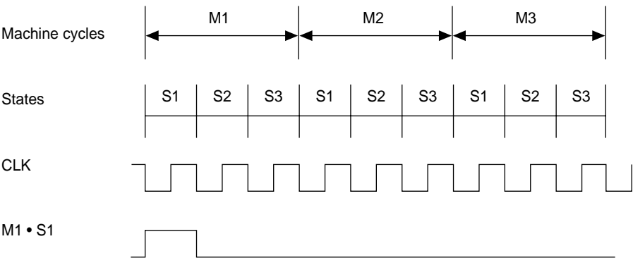
Figure 1-5 Machine Cycle Definition
