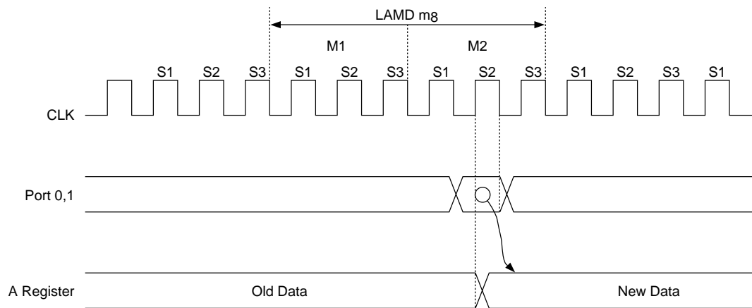
Figure 7-4 Example of Reading the Data from the Port by the "LAMD m8" Instruction
