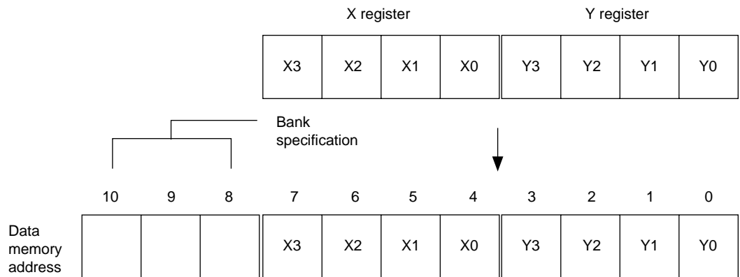
Figure 2-8 Data Memory Address of XY Indirect Addressing
