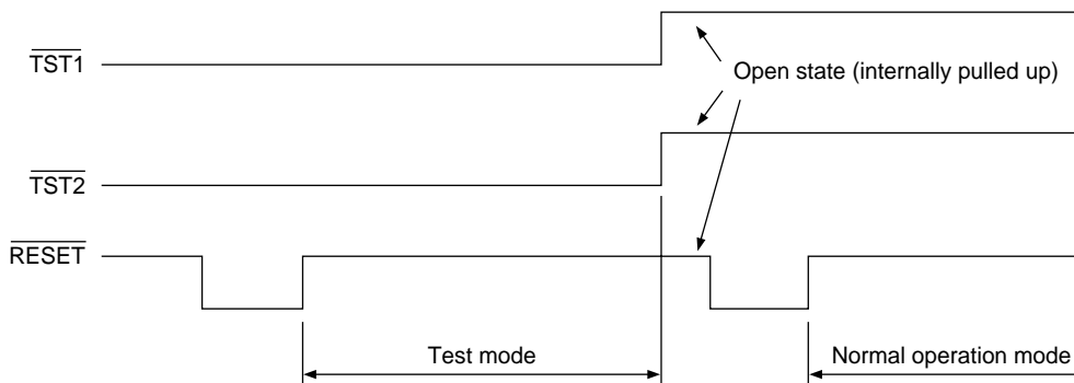
Figure 15-1 Relation among the \overline{TST1} , \overline{TST2} pins and the \overline{RESET} pin
