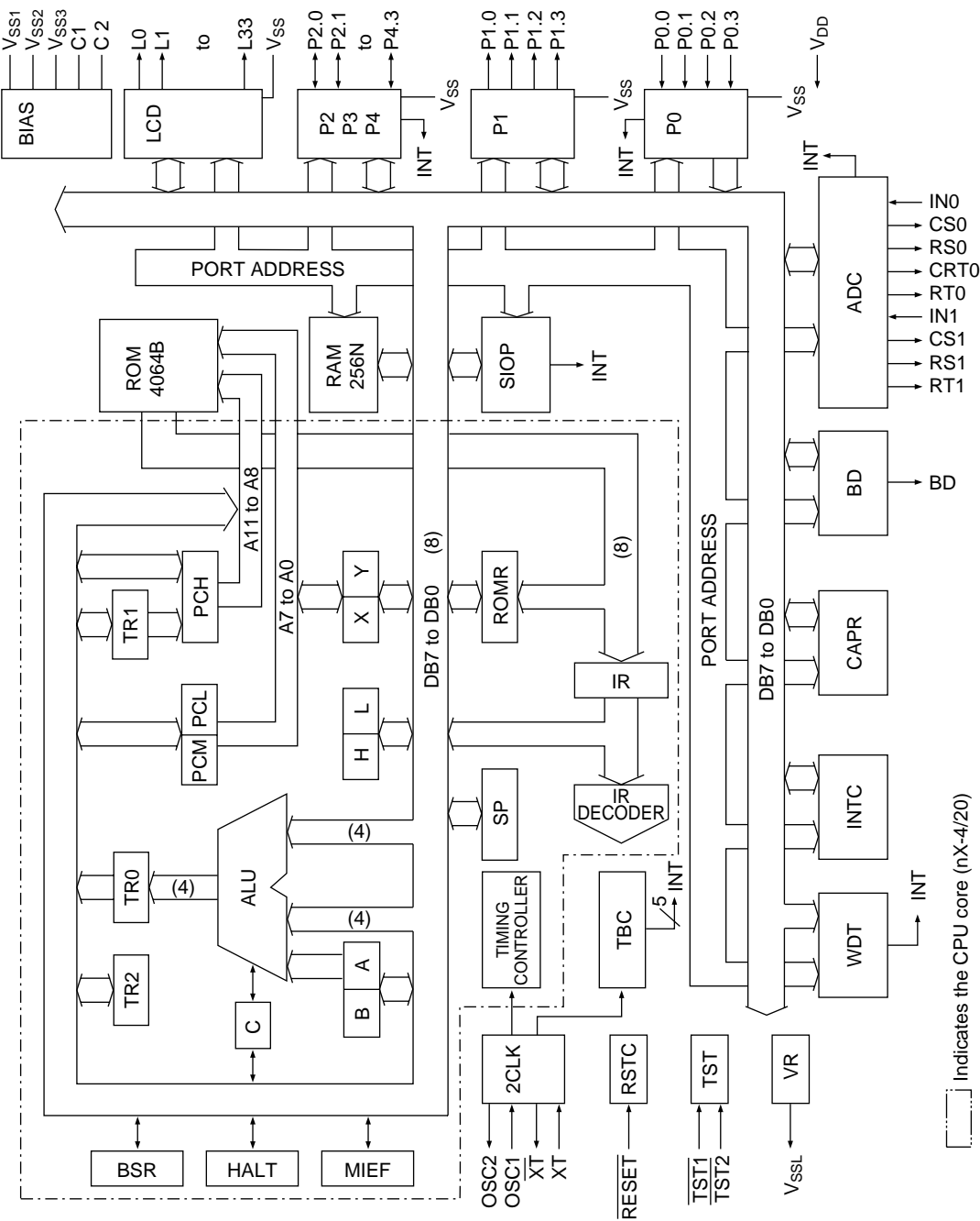
Figure 1-1 MSM64164C Block Diagram
