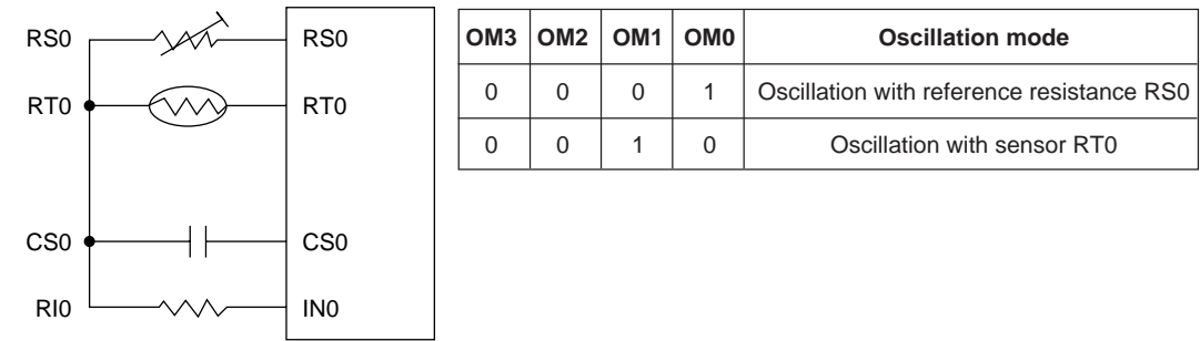
Figure 12-2 Measurement of CROSC0 by a Resistance Sensor
