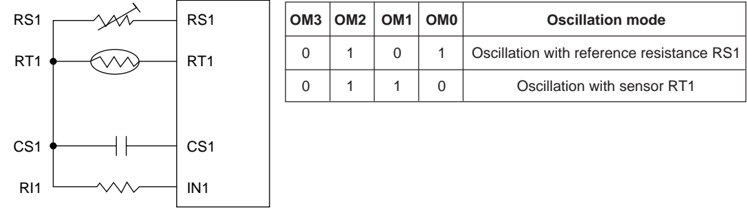
Figure 12-5 Measurement of CROSC1 by a Resistance Sensor
