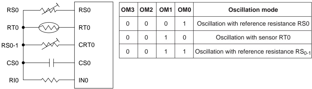
Figure 12-3 Measurement of CROSC0 by a Resistance Sensor (when two-point adjustment with two reference resistances)
