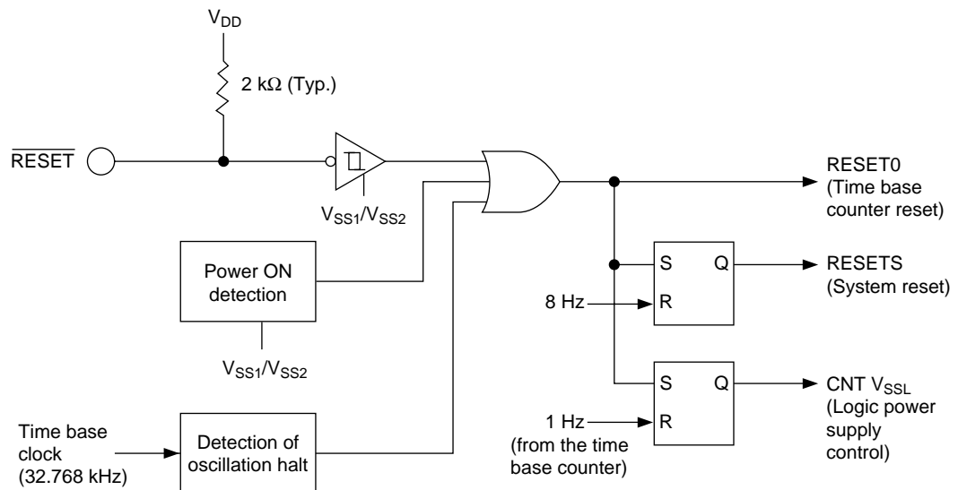
Figure 3-2 System Reset Generation Circuit
