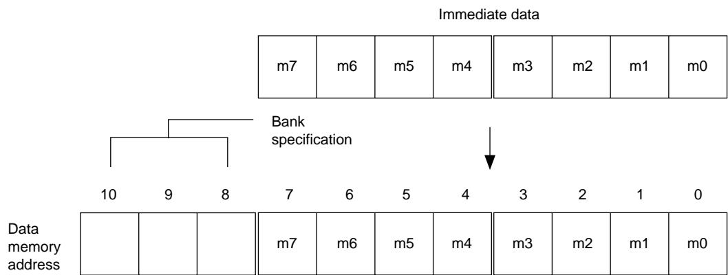
Figure 2-9 Data Memory Address of Direct Addressing
