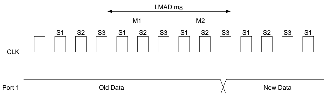
Figure 7-3 Example of Writing to Port Data Register by "LMAD m8" Instruction
