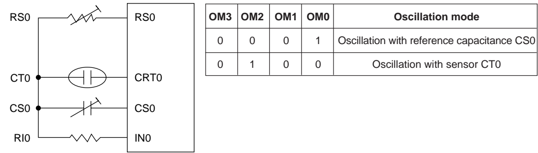
Figure 12-4 Measurement of CROSC0 by a Capacitance Sensor
