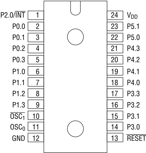
24-Pin Plastic DIP
