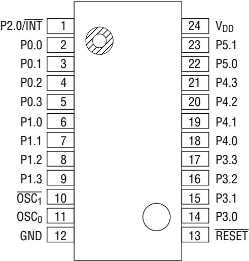
24-Pin Plastic SOP
