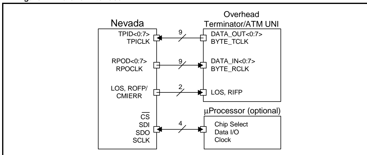
Figure 12. Parallel Interface
