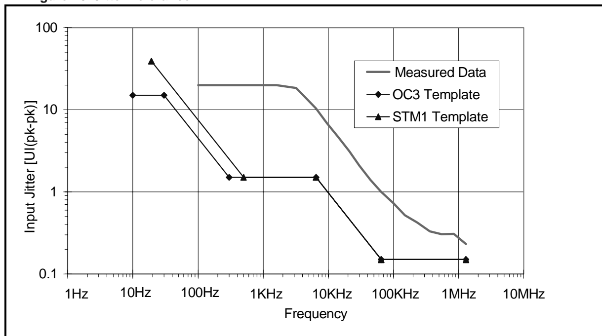
Figure 26. Jitter Tolerance
