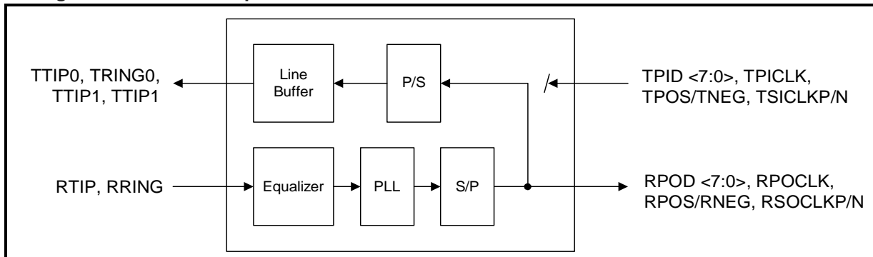
Figure 14. Remote Loopback
