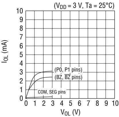
Low-level Output Current ( I_{OL} ) - Output Voltage ( V_{OL} )
