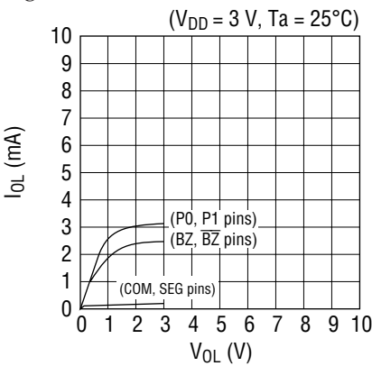
Low-level Output Current ( I_{OL} ) - Output Voltage ( V_{OL} )
