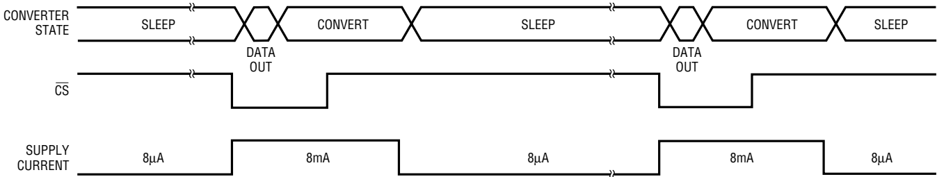
Figure 15. Reduced Power Timing Mode
