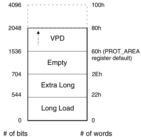
Figure 4-5. Serial EEPROM Memory Map
