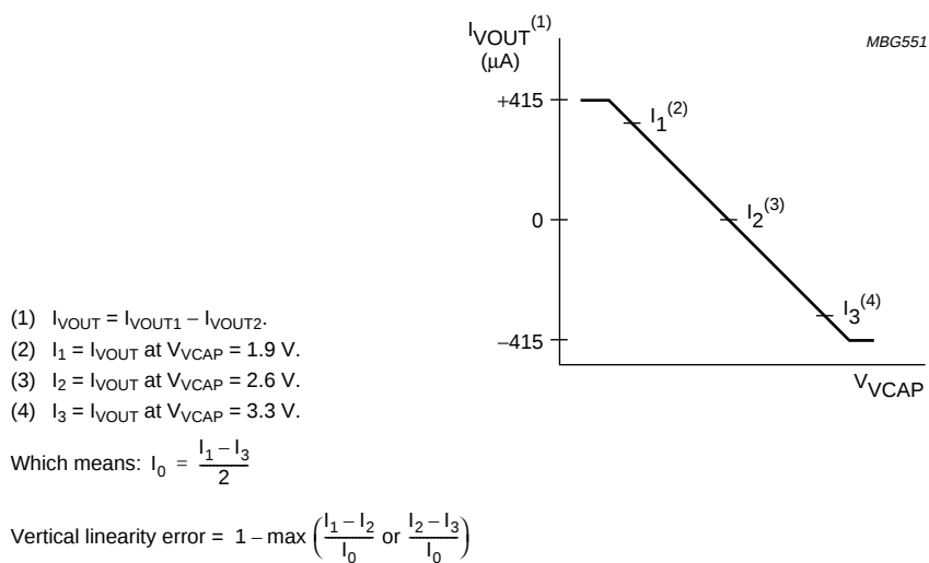
Fig.27 Definition of vertical linearity error.
