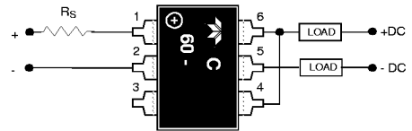
B) DC CONFIGURATION (SEE NOTE 4)
