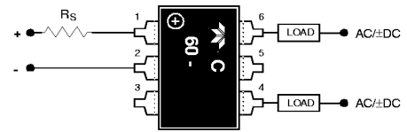
A) BI-DIRECTIONAL/AC CONFIGURATION (SEE NOTE 4)
