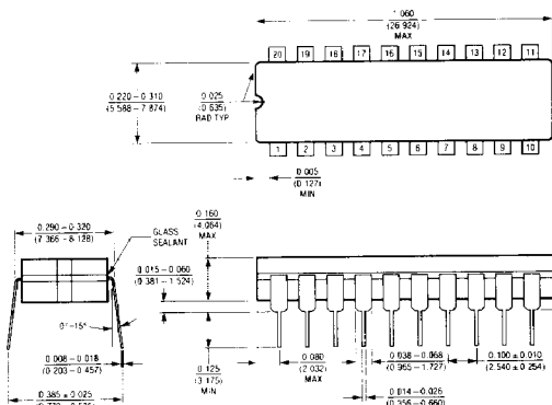
J Package 20 Lead Ceramic DIP
