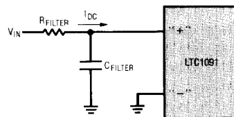
Figure 11. RC Input Filtering
