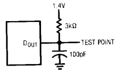
Load Circuit for t_{dO} , t_r , and t_f
