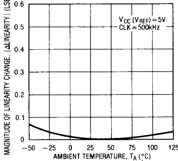
Change in Linearity Error vs Temperature
