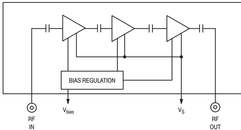
Figure 1. Internal Diagram
