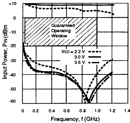
FREQUENCY RESPONSE (DIVIDE-BY-8 @ T_A = 25^\circ\text{C} )
