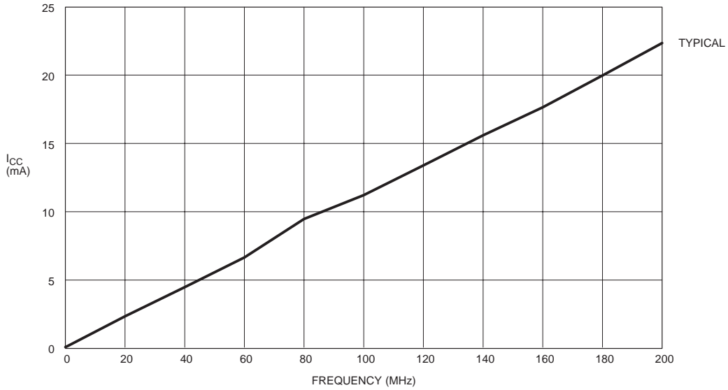
Figure 5: I_{CC} vs. Frequency at V_{CC} = 3.3\text{ V} , 25^\circ\text{C}
