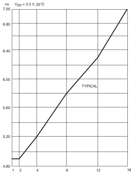
Figure 6: t_{PD\_PAL} vs. Output Switching
