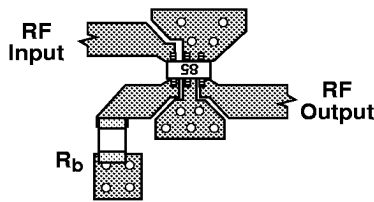
Figure 18. RF Layout.
