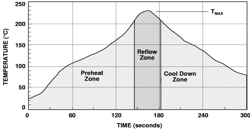
Figure 26. Surface Mount Assembly Profile.
