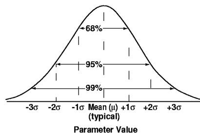
Figure 24. Normal Distribution.
