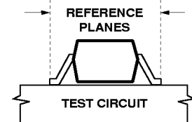
Figure 25. Phase Reference Planes.
