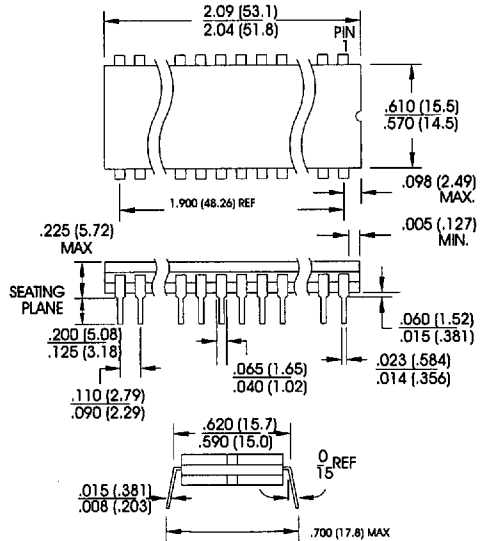
40D6 , 40 Lead, 0.600" Wide, Non-Windowed, Ceramic Dual Inline Package (Cerdip) Dimensions in Inches and (Millimeters) MIL-STD-1835 D-5 CONFIG A
