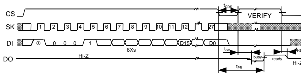
Figure 19 WRAL Timing (S-29330A)
