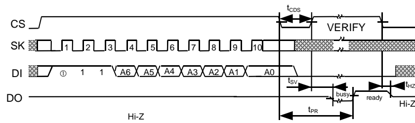
Figure 13 ERASE Timing (S-29230A)
