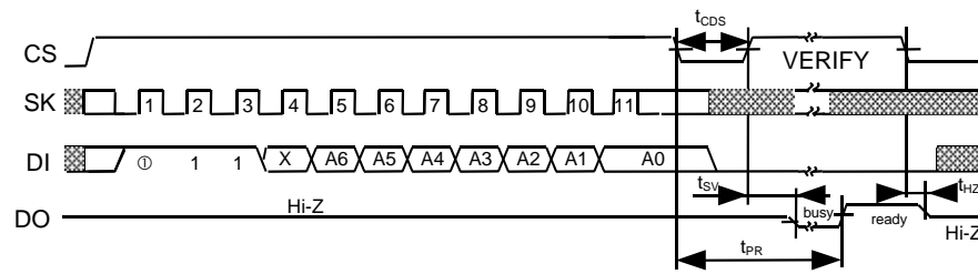
Figure 14 ERASE Timing (S-29220A)
