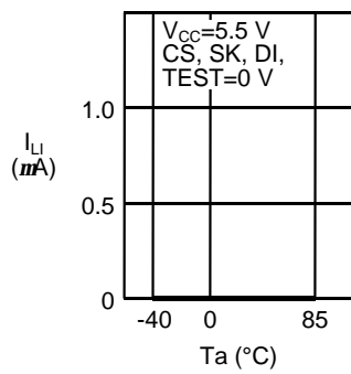
1.11 Input leakage current I_{LI} – Ambient temperature T_a
