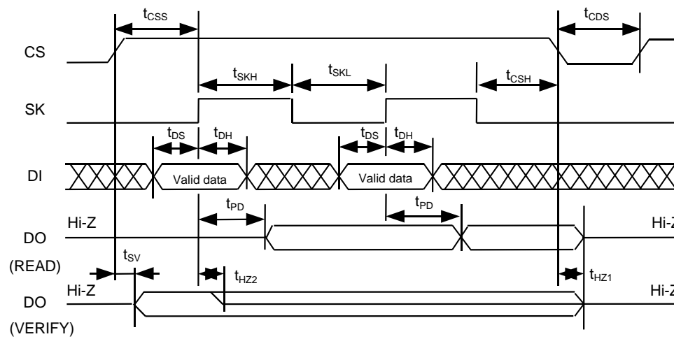
Figure 3 Timing Chart
