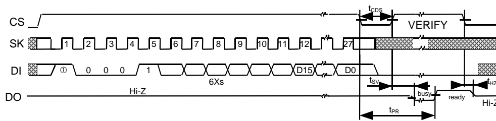
Figure 18 WRAL Timing (S-29220A)
