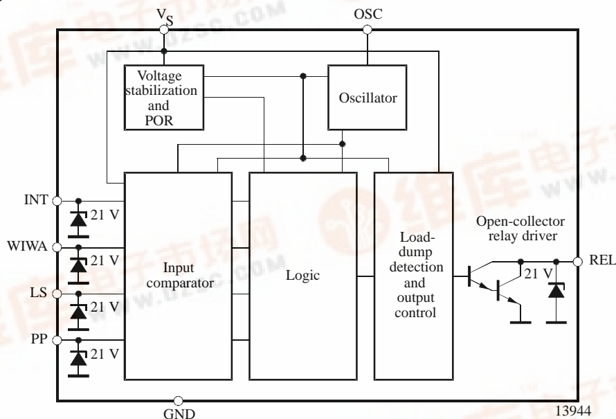
Figure 1. Block diagram
