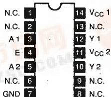
NTE75322 14-Lead DIP, See Diag. 247
