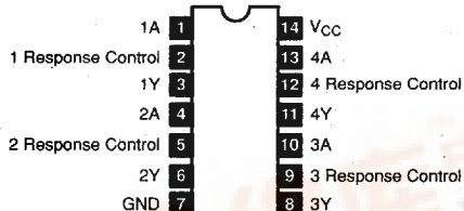
NTE75189 14-Lead DIP, See Diag. 247
