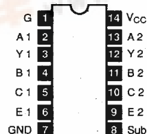
NTE75450B 14-Lead DIP, See Diag. 247
