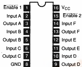
NTE6885, NTE6886 16-Lead DIP, See Diag. 249
