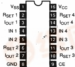
NTE75493 16-Lead DIP, See Diag. 249
