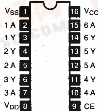
NTE75494 16-Lead DIP, See Diag. 249
