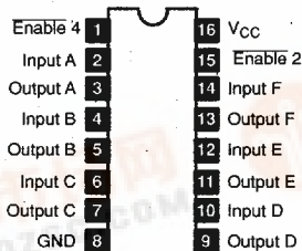
NTE6887, NTE6888 16-Lead DIP, See Diag. 249
