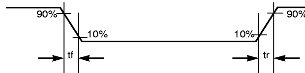
Figure 1. Switching Characteristics
