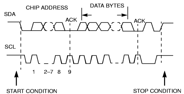
Figure 2. M_BUS Format
