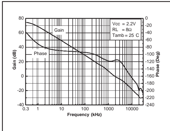
Fig. 7 : Open Loop Frequency Response
