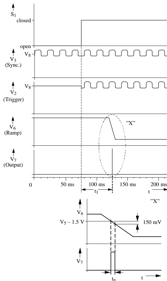
Figure 3. Signal characteristics
