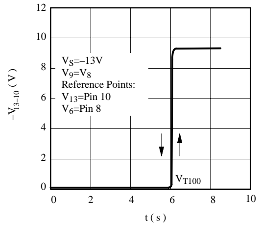
Figure 14. Overload switching
