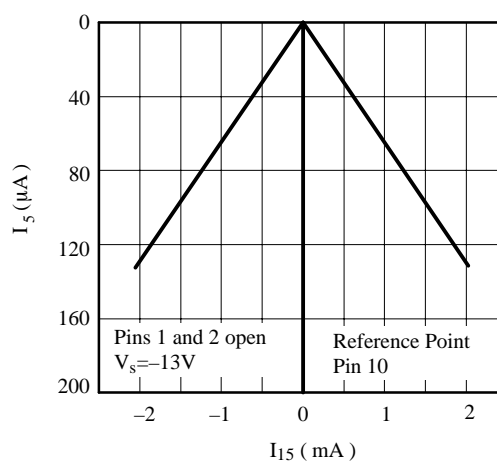
Figure 9. Soft-start characteristic
