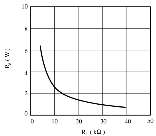
Figure 15. Load limitation
