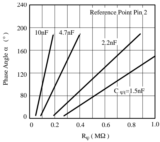
Figure 6. Ramp control
