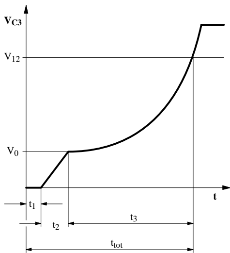
Figure 4. Soft start
