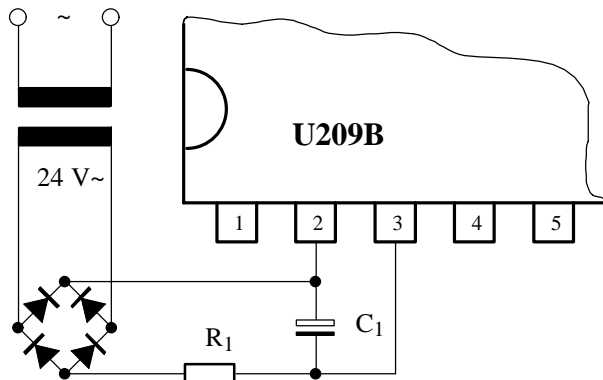
Figure 3. Supply voltage for high current requirements
